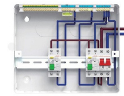
DUAL RCD / HIGH INTEGRITY
