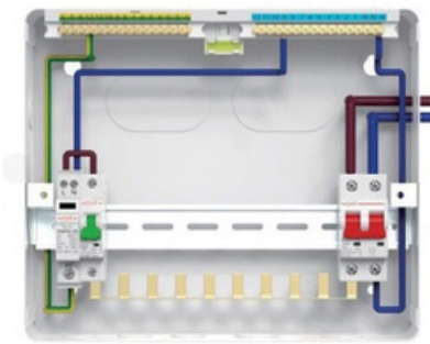
MAIN SWITCH and SPD
